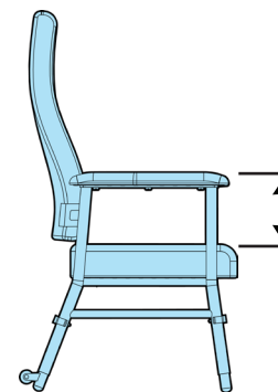
Armrest height Armrest to top of seat 220mm (H)
