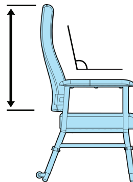
Backrest height & angle 700mm (H) x 98°
