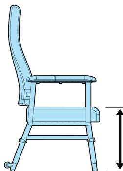
Seat height Floor to top of seat 450mm 525mm 475mm 550mm 500mm 575mm
