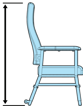
Overall height (at lowest setting) 1160mm (H)
